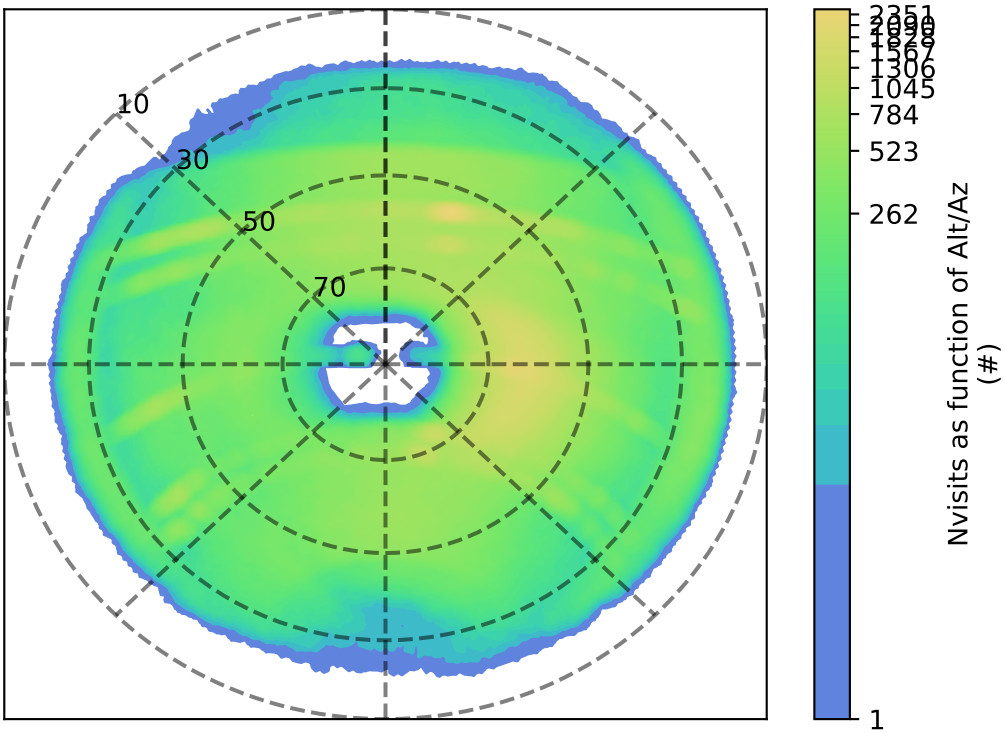
roll_uniform_eh_acc0.5_mjdp0_v3.4_10yrs z: Nvisits as function of Alt/Az
