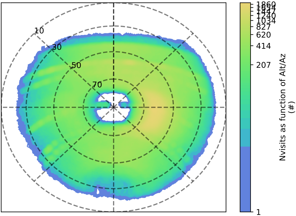
roll_uniform_eh_acc0.5_mjdp0_v3.4_10yrs y: Nvisits as function of Alt/Az
