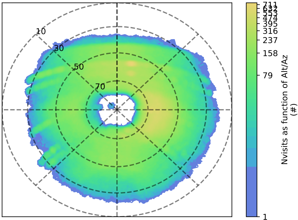
roll_uniform_eh_acc0.5_mjdp0_v3.4_10yrs u: Nvisits as function of Alt/Az
