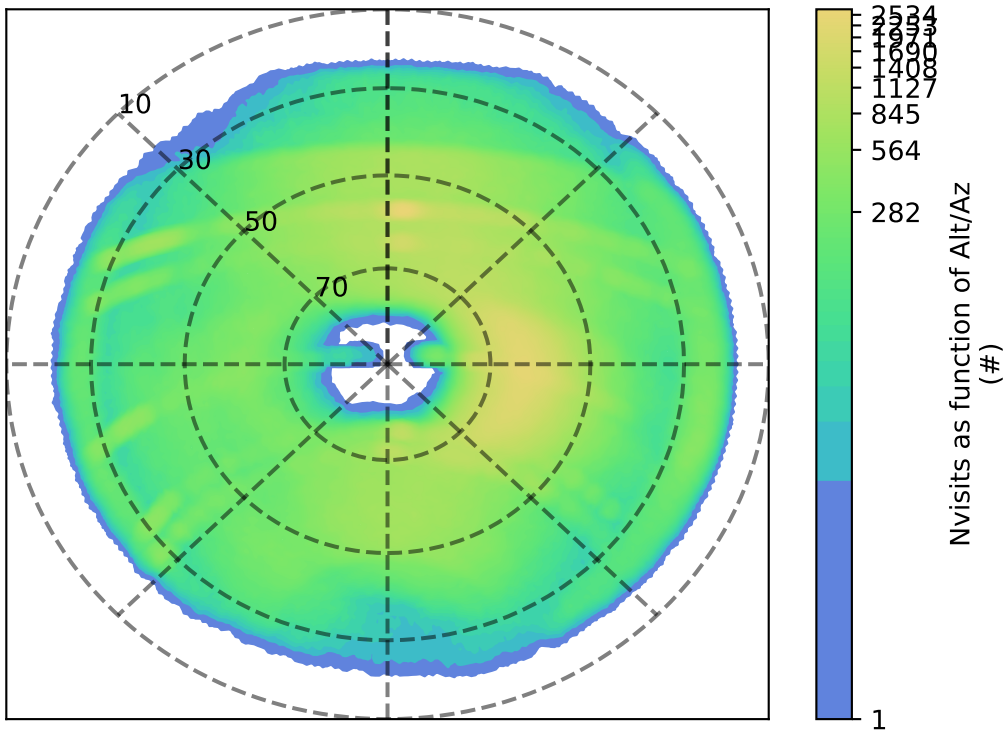
roll_uniform_eh_acc0.5_mjdp0_v3.4_10yrs i: Nvisits as function of Alt/Az
