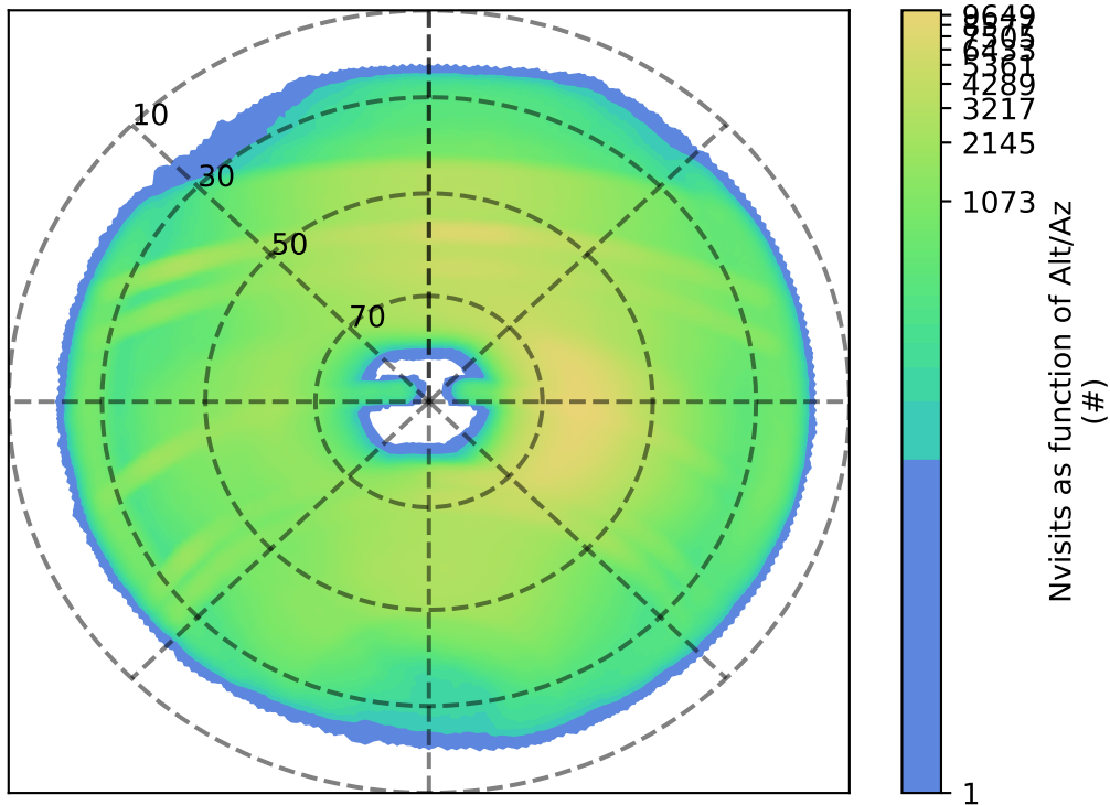
roll_uniform_eh_acc0.5_mjdp0_v3.4_10yrs : Nvisits as function of Alt/Az
