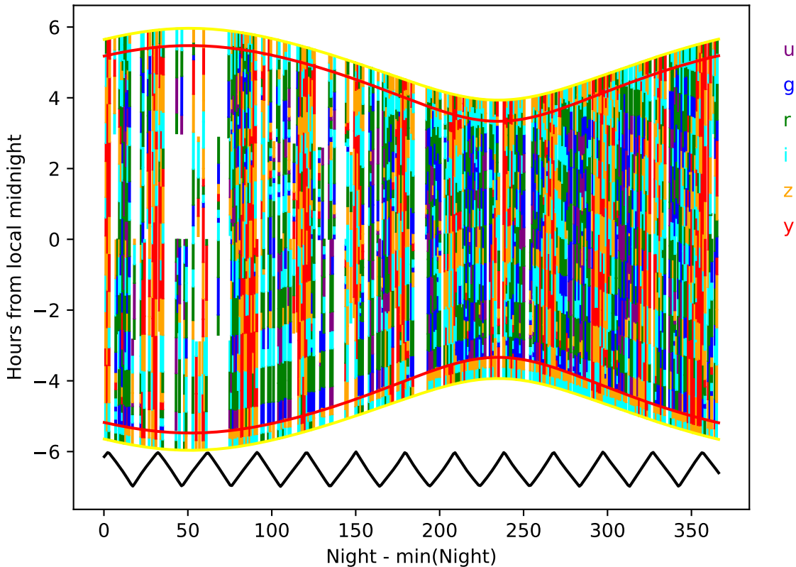
roll_uniform_eh_acc0.5_mjdp0_v3.4_10yrs year 9-10: Hourglass
