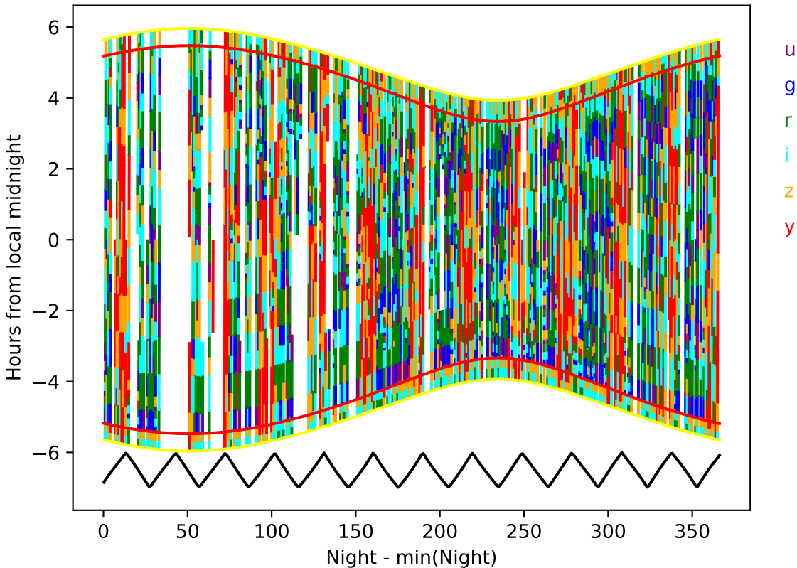
roll_uniform_eh_acc0.5_mjdp0_v3.4_10yrs year 8-9: Hourglass
