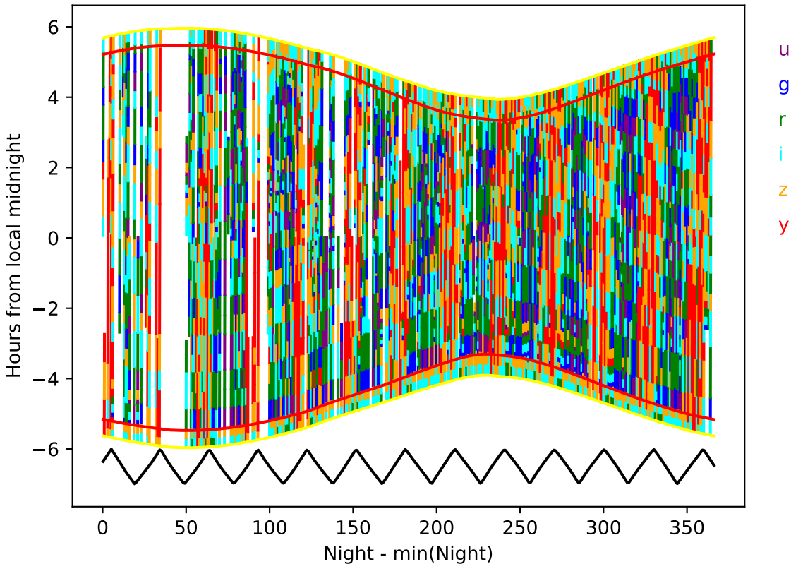
roll_uniform_eh_acc0.5_mjdp0_v3.4_10yrs year 6-7: Hourglass
