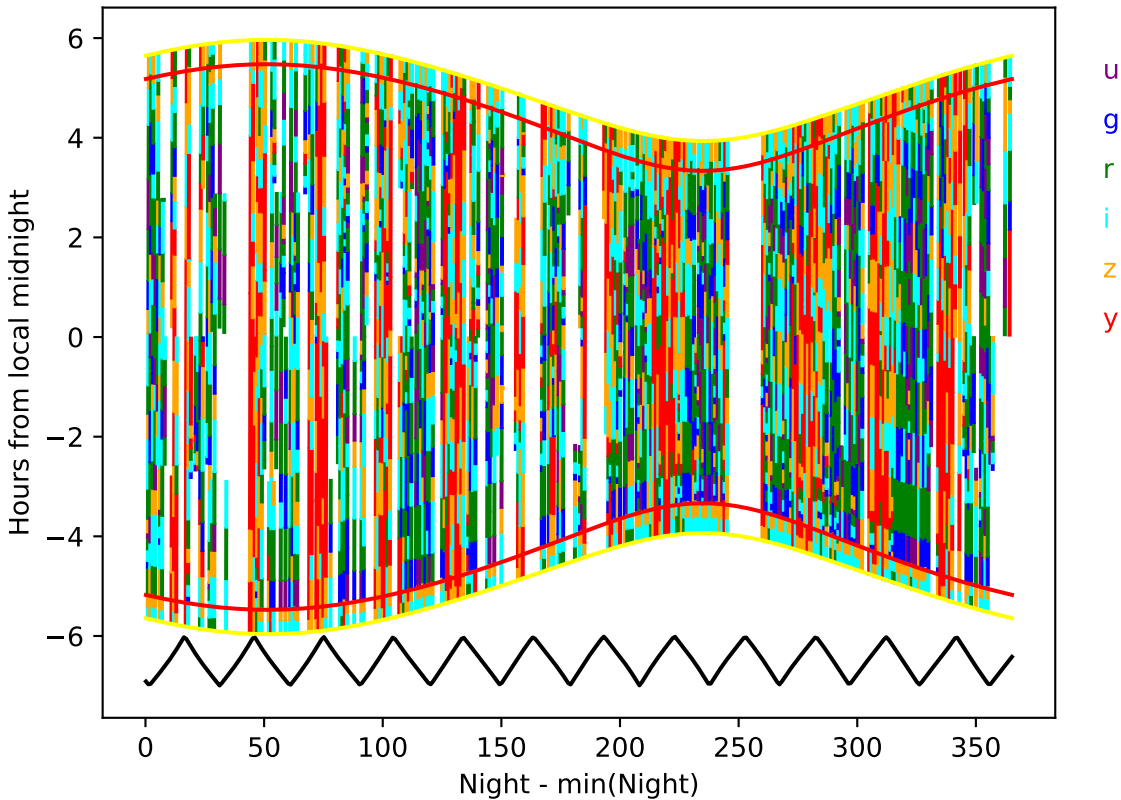
roll_uniform_eh_acc0.5_mjdp0_v3.4_10yrs year 5-6: Hourglass
