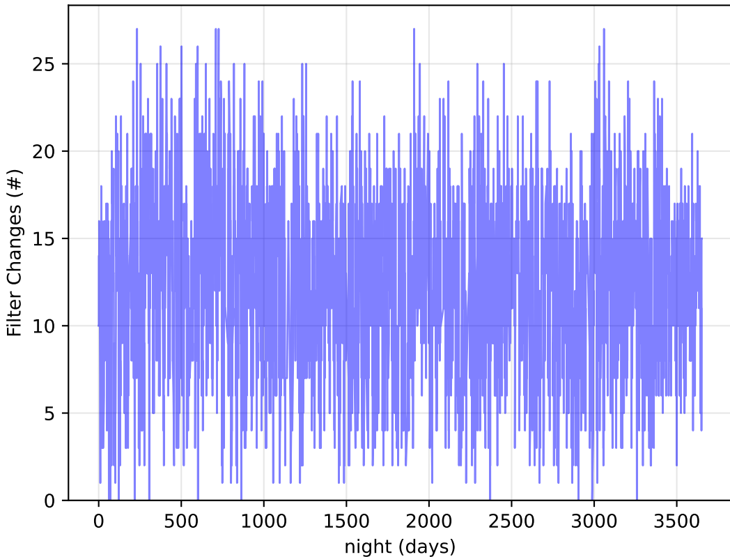
roll_uniform_eh_acc0.5_mjdp0_v3.4_10yrs : Filter Changes
