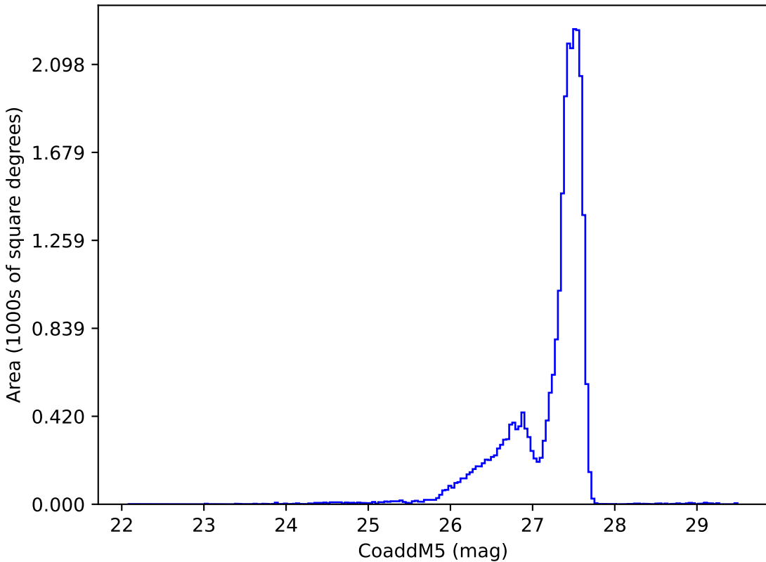
roll_uniform_eh_acc0.5_mjdp0_v3.4_10yrs : CoaddM5
