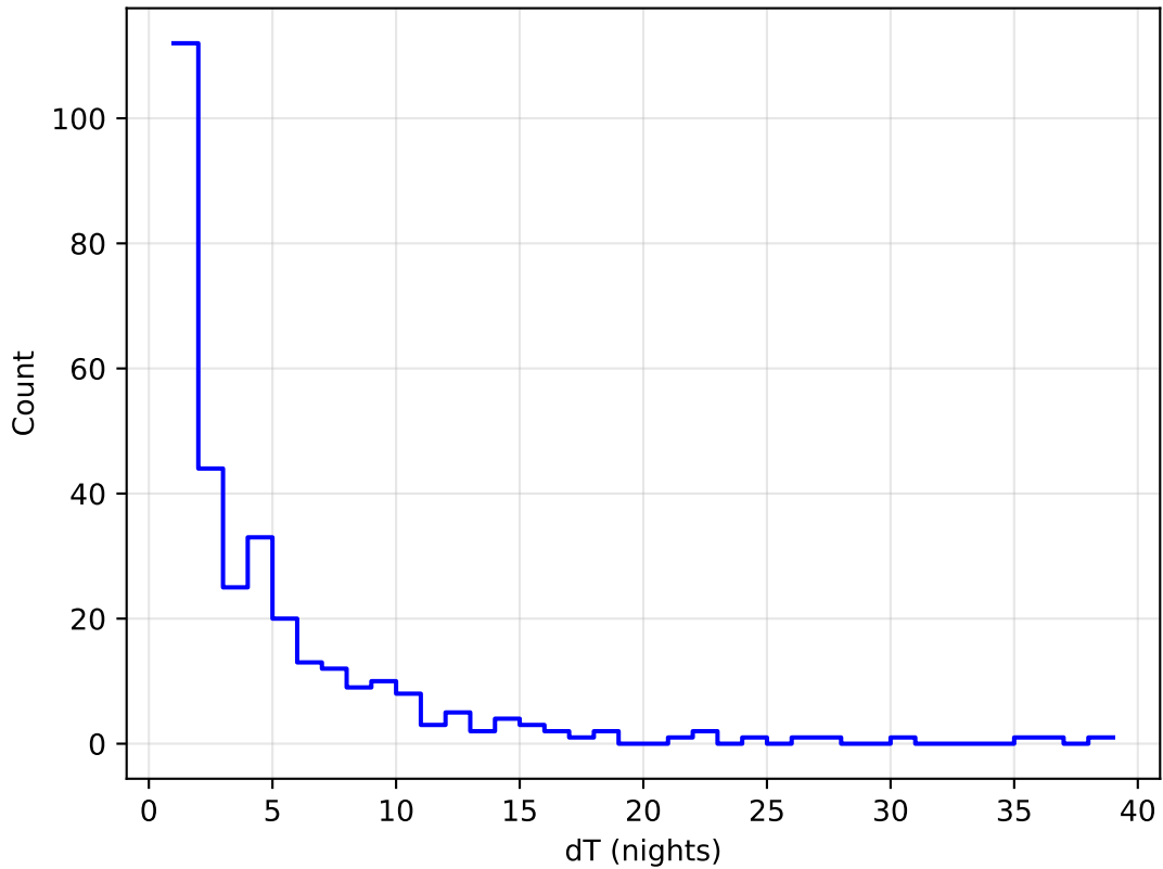
roll_uniform_eh_acc0.5_mjdp0_v3.4_10yrs all bands: DD:WFD Delta Nights Histogram
