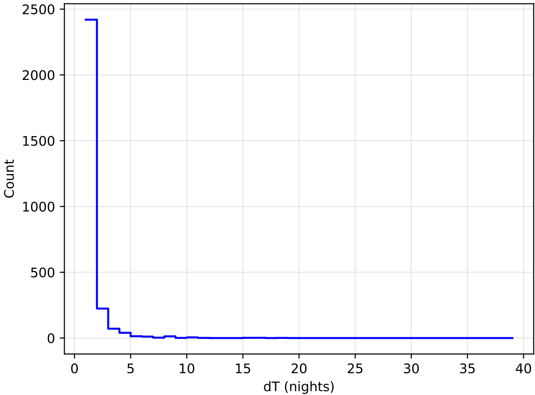
roll_uniform_eh_acc0.5_mjdp0_v3.4_10yrs all bands: DD:WFD Delta Nights Histogram
