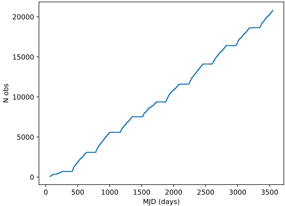
roll_uniform_eh_acc0.5_mjdp0_v3.4_10yrs all bands: DD:ELAISS1 Cumulative NVisits
