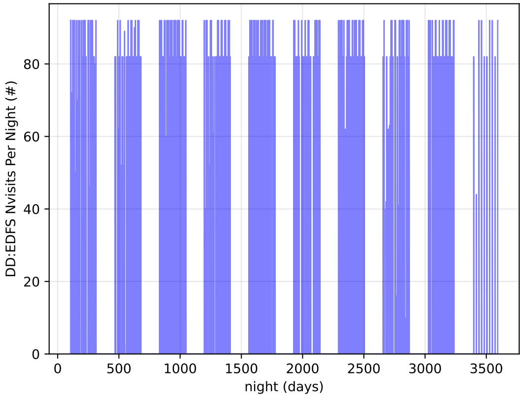
roll_uniform_eh_acc0.5_mjdp0_v3.4_10yrs all bands: DD:EDFS Nvisits Per Night
