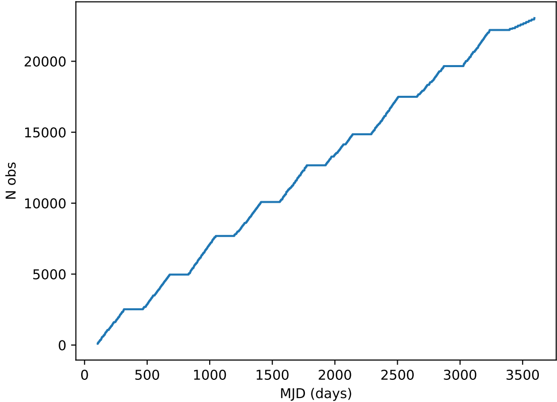
roll_uniform_eh_acc0.5_mjdp0_v3.4_10yrs all bands: DD:EDFS Cumulative NVisits
