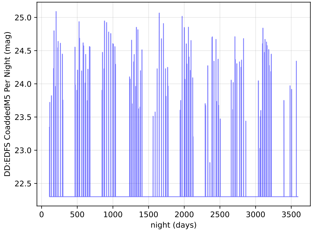
roll_uniform_eh_acc0.5_mjdp0_v3.4_10yrs u band: DD:EDFS CoaddedM5 Per Night
