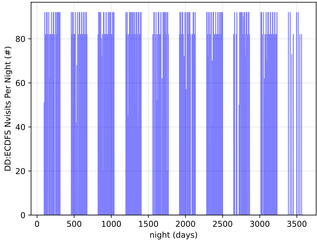
roll_uniform_eh_acc0.5_mjdp0_v3.4_10yrs all bands: DD:ECDFS Nvisits Per Night
