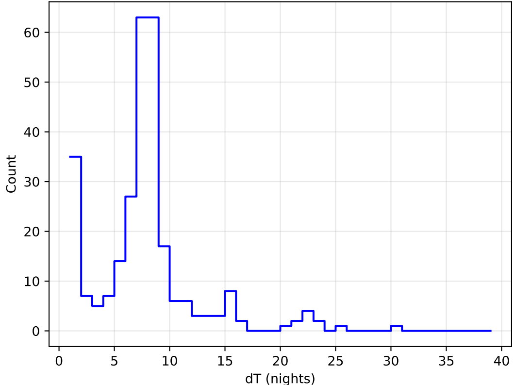
roll_uniform_eh_acc0.5_mjdp0_v3.4_10yrs all bands: DD:ECDFS Delta Nights Histogram
