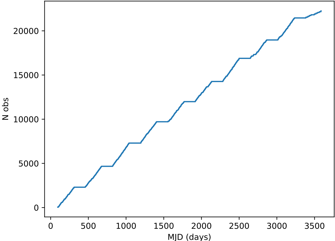
roll_uniform_eh_acc0.5_mjdp0_v3.4_10yrs all bands: DD:ECDFS Cumulative NVisits
