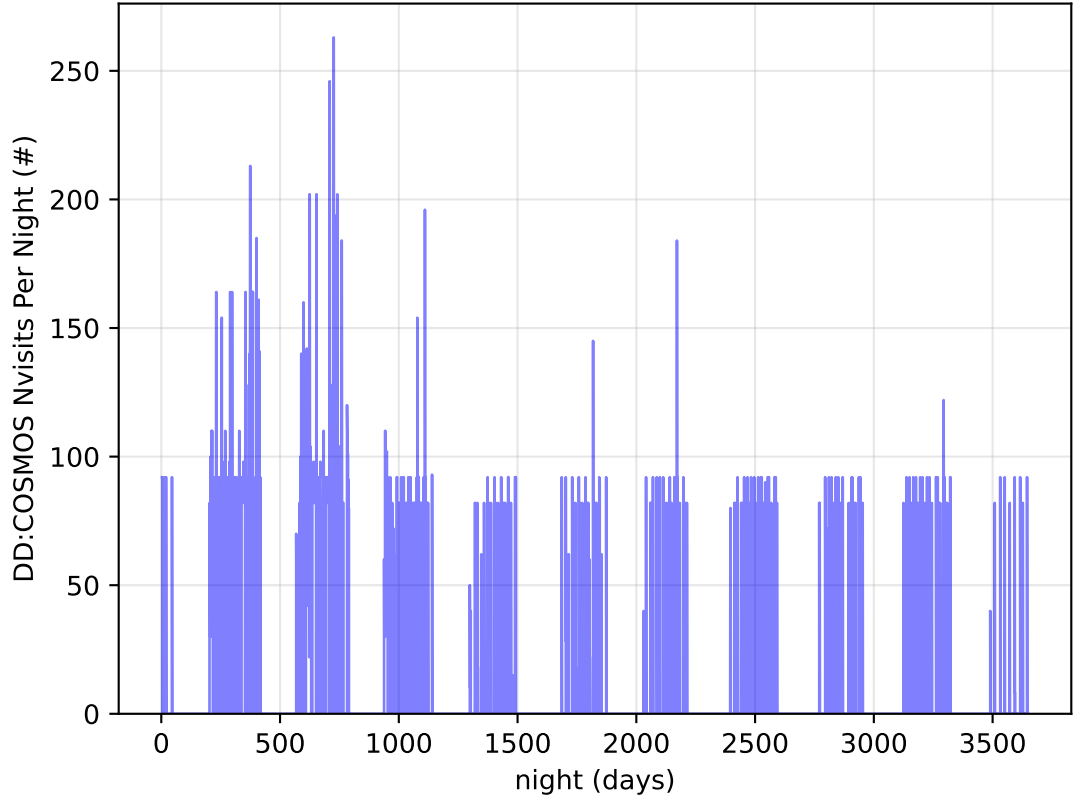
roll_uniform_eh_acc0.5_mjdp0_v3.4_10yrs all bands: DD: COSMOS Nvisits Per Night
