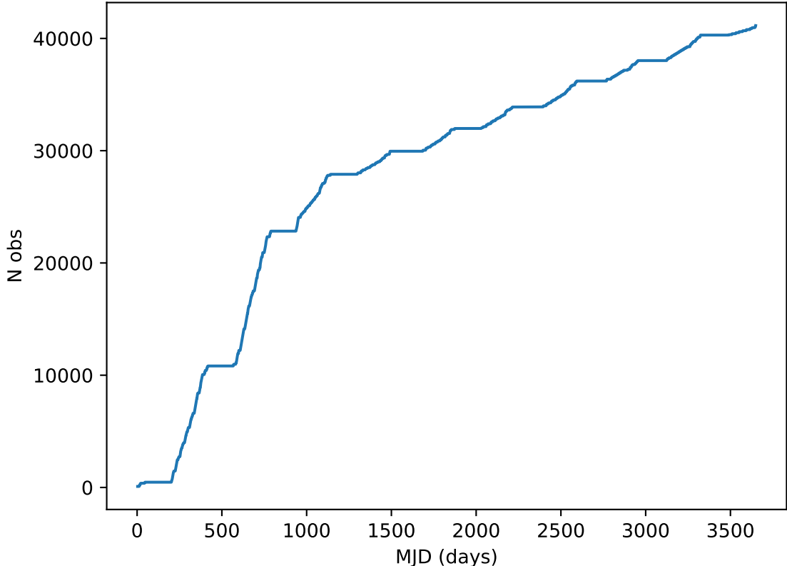
roll_uniform_eh_acc0.5_mjdp0_v3.4_10yrs all bands: DD: COSMOS Cumulative NVisits
