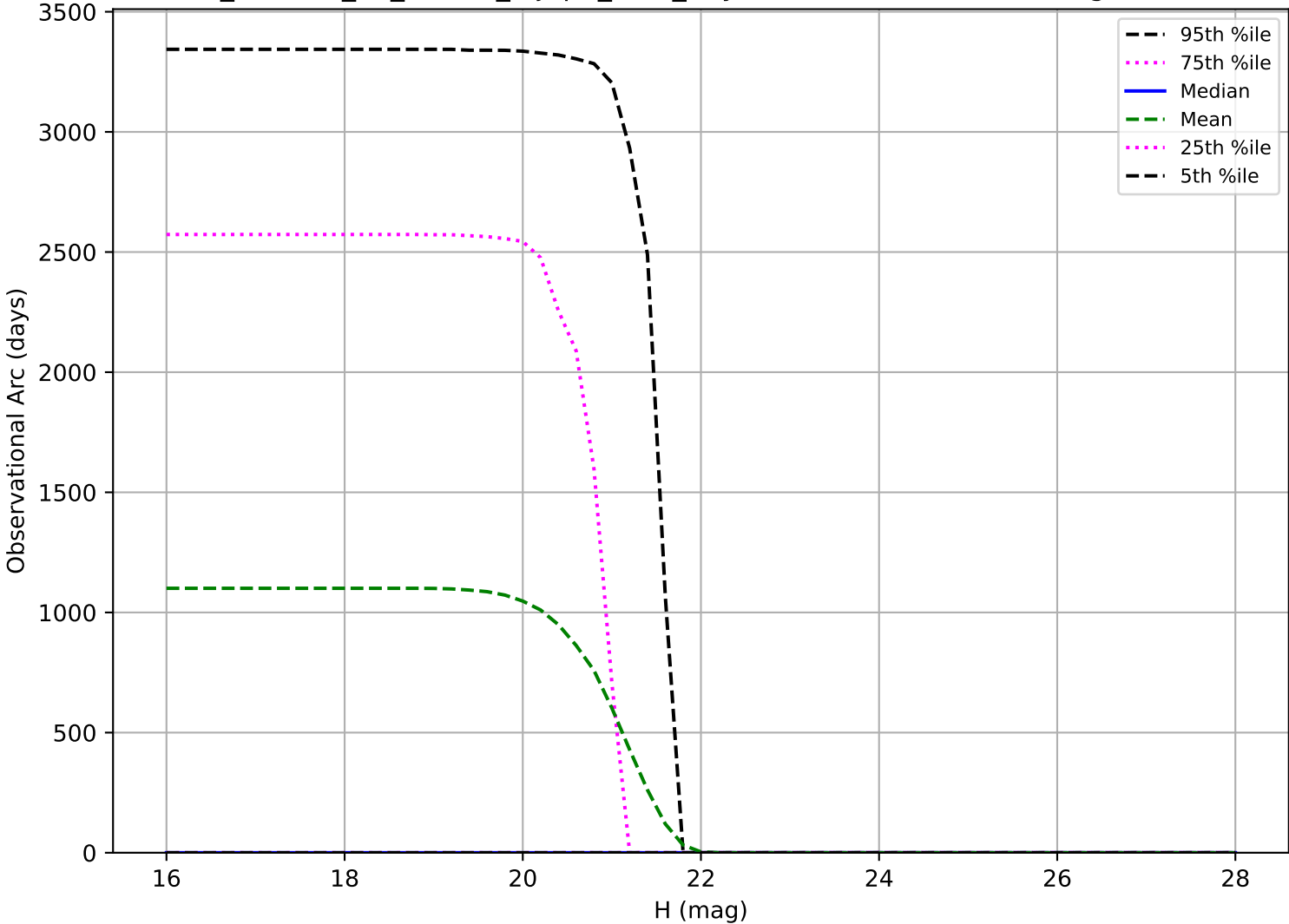
roll_uniform_eh_acc0.2_mjdp0_v3.4_10yrs: Observational Arc Length Vatira
