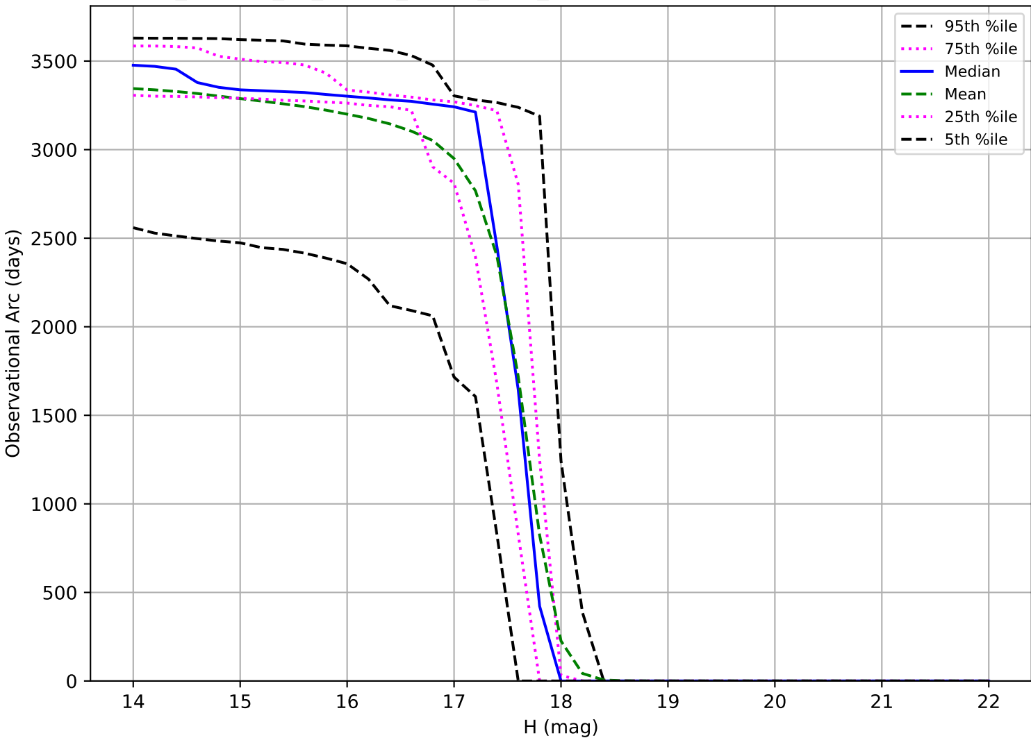
roll_uniform_eh_acc0.2_mjdp0_v3.4_10yrs: Observational Arc Length Trojan
