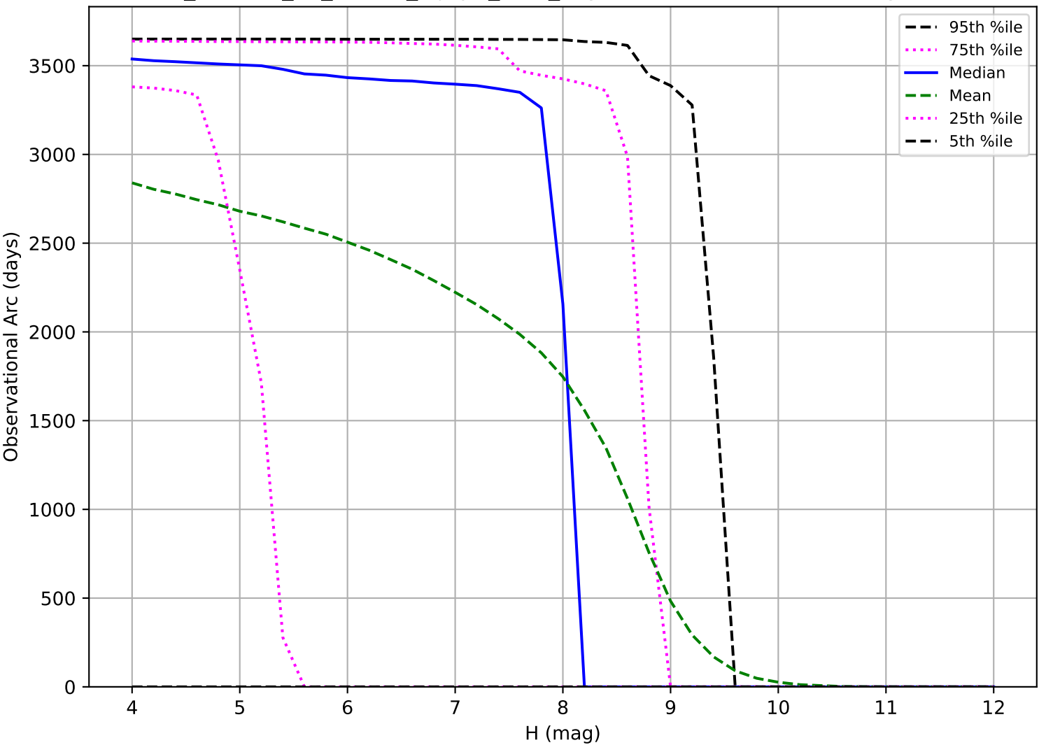
roll_uniform_eh_acc0.2_mjdp0_v3.4_10yrs: Observational Arc Length TNO
