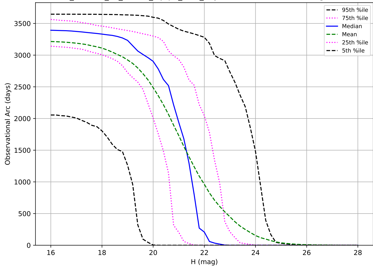
roll_uniform_eh_acc0.2_mjdp0_v3.4_10yrs: Observational Arc Length PHA
