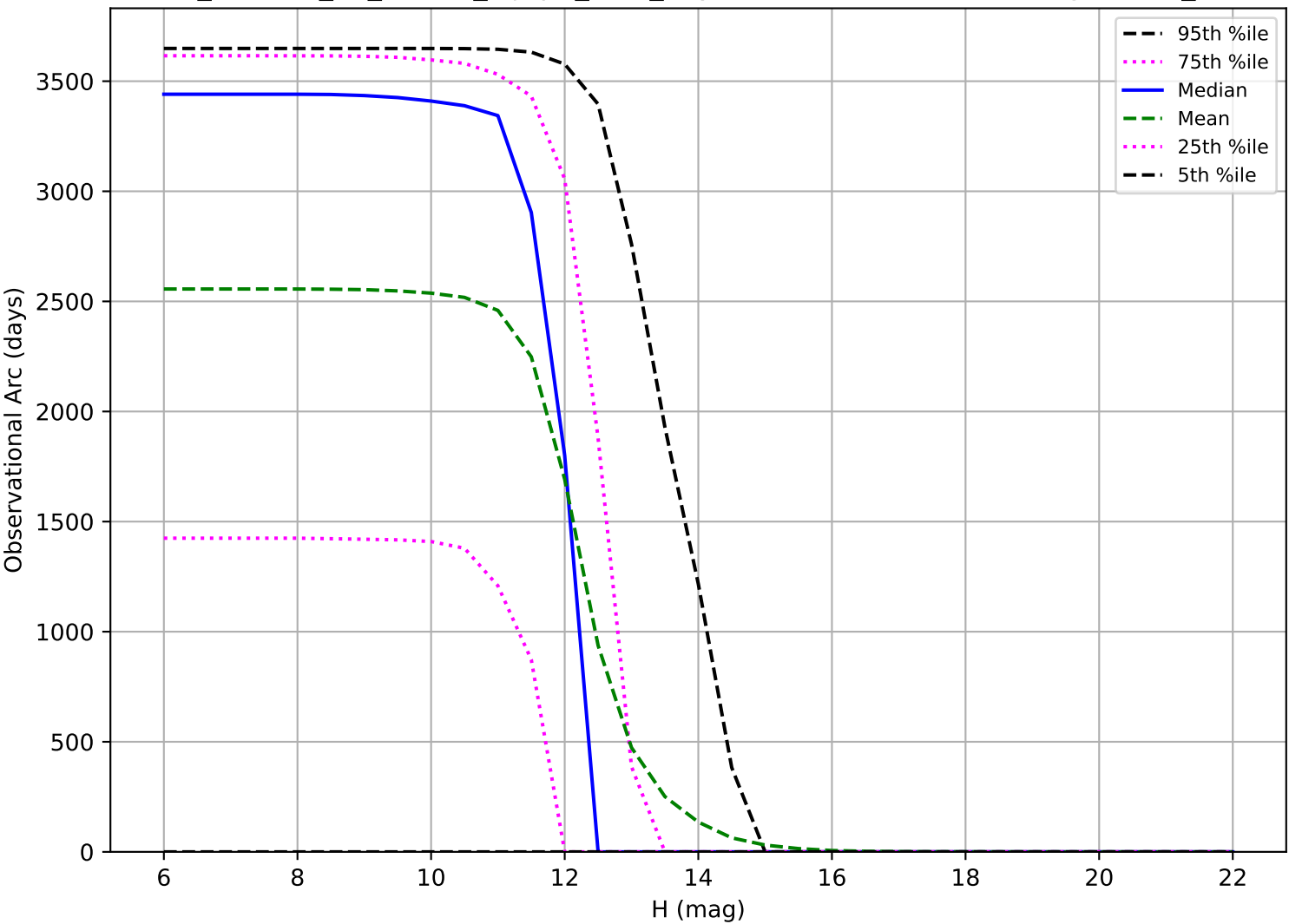
roll_uniform_eh_acc0.2_mjdp0_v3.4_10yrs: Observational Arc Length OCC_r20
