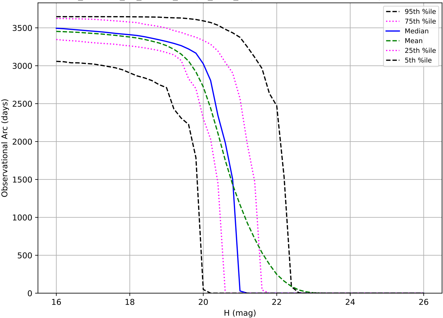
roll_uniform_eh_acc0.2_mjdp0_v3.4_10yrs: Observational Arc Length MBA
