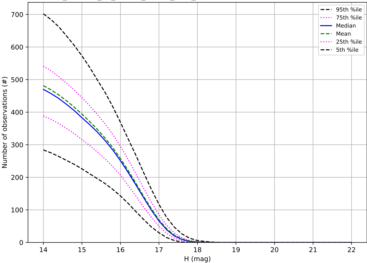
roll_uniform_eh_acc0.2_mjdp0_v3.4_10yrs: Number of observations Trojan
