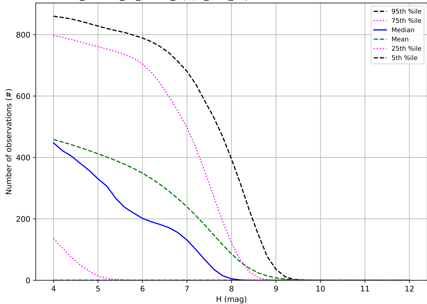
roll_uniform_eh_acc0.2_mjdp0_v3.4_10yrs: Number of observations TNO
