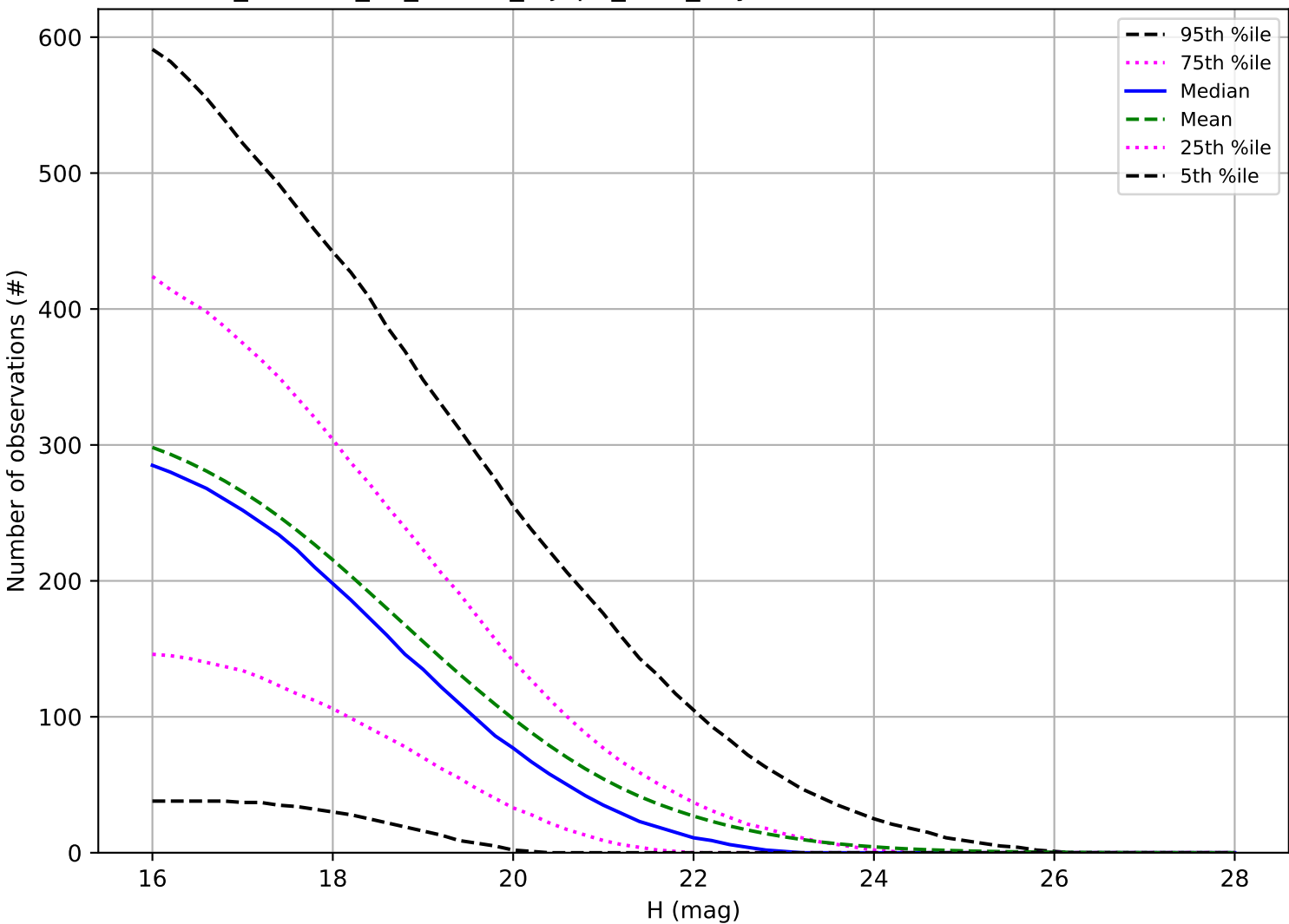
roll_uniform_eh_acc0.2_mjdp0_v3.4_10yrs: Number of observations PHA
