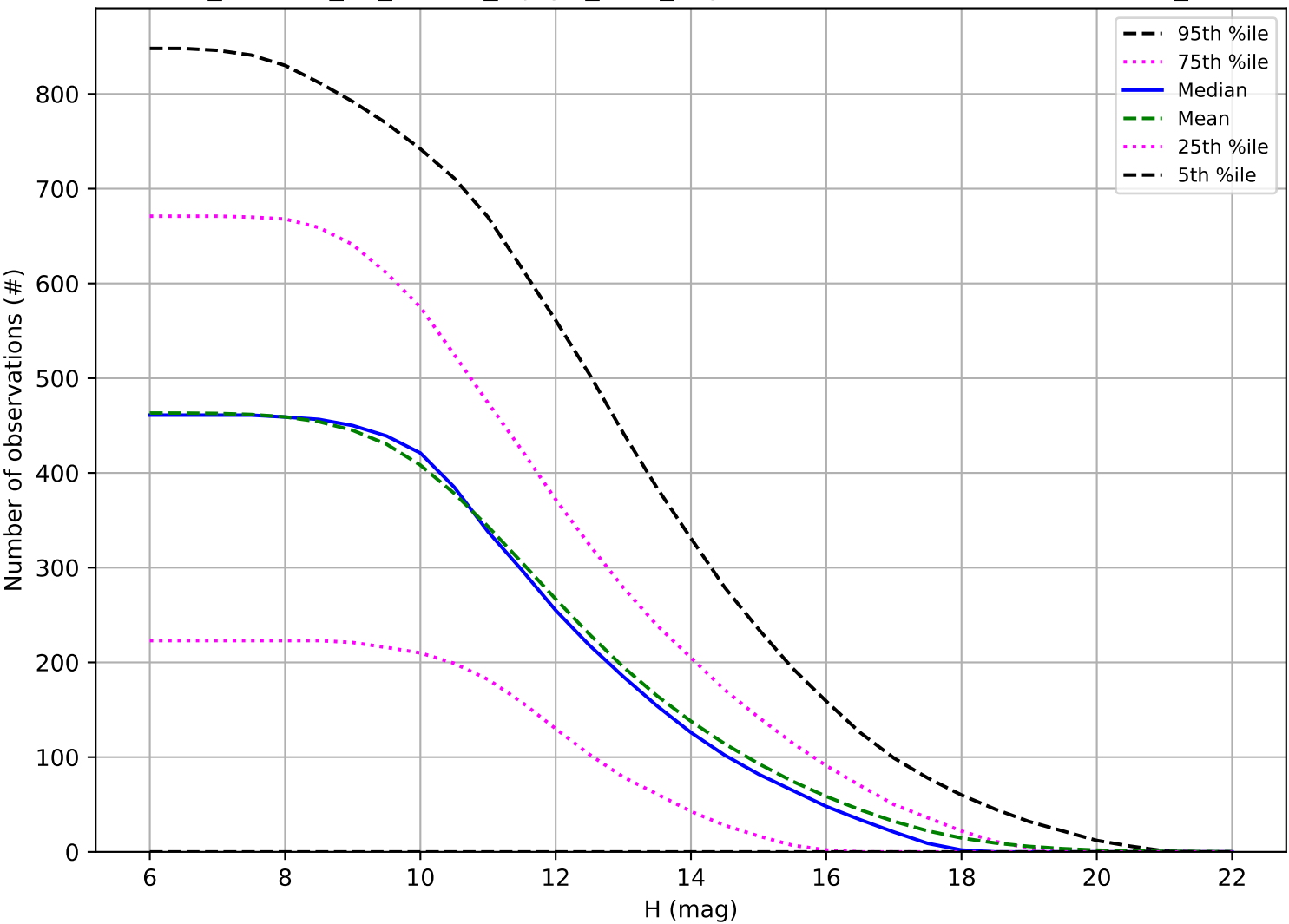
roll_uniform_eh_acc0.2_mjdp0_v3.4_10yrs: Number of observations OCC_r5
