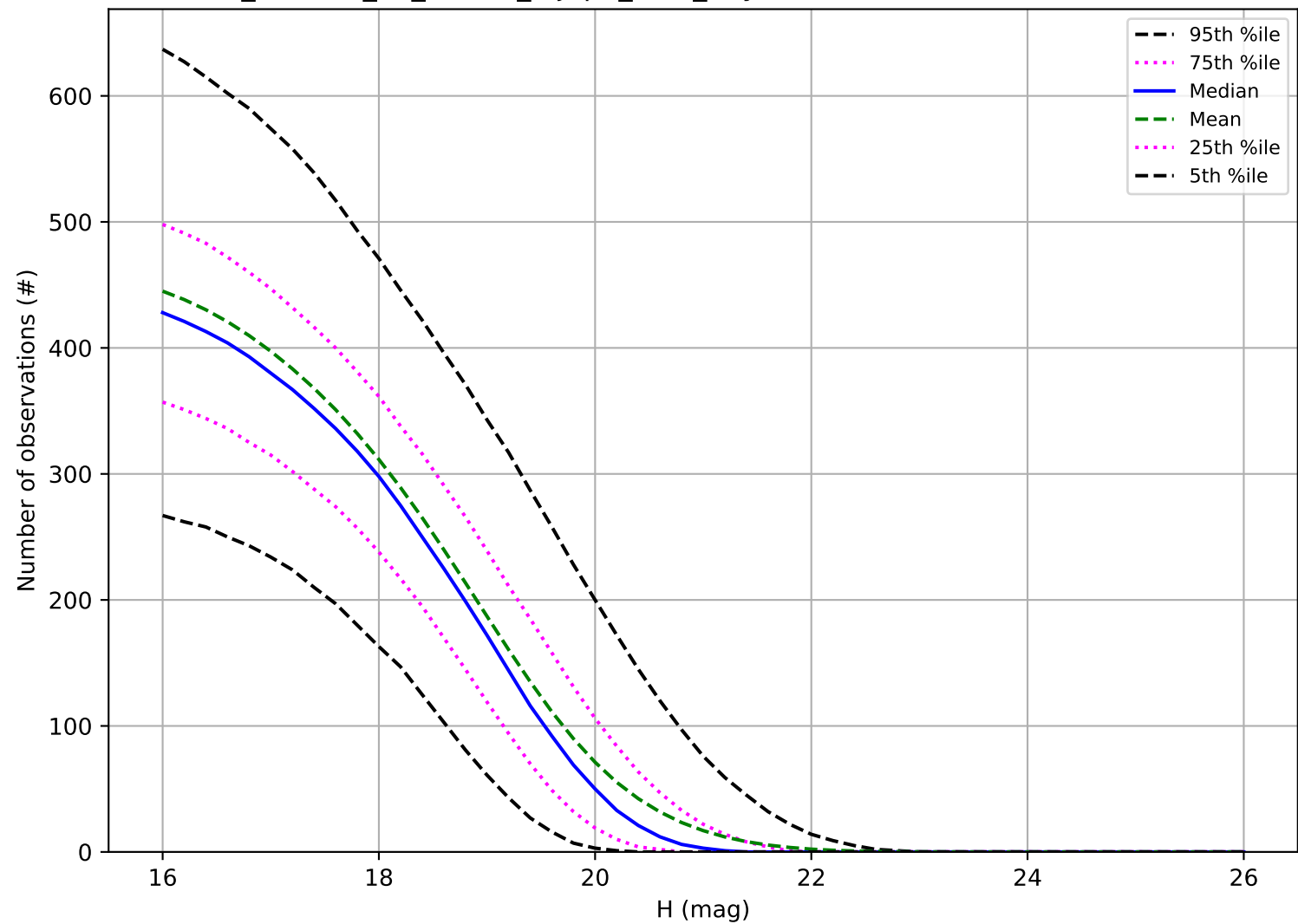
roll_uniform_eh_acc0.2_mjdp0_v3.4_10yrs: Number of observations MBA
