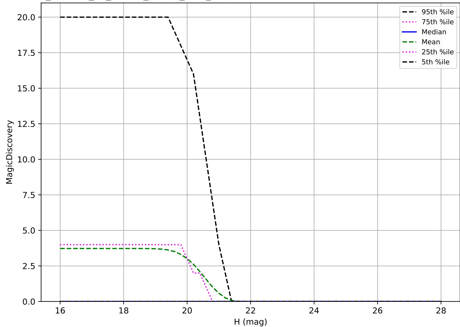
roll_uniform_eh_acc0.2_mjdp0_v3.4_10yrs: Vatira 6 detections in 60 nights detection loss
