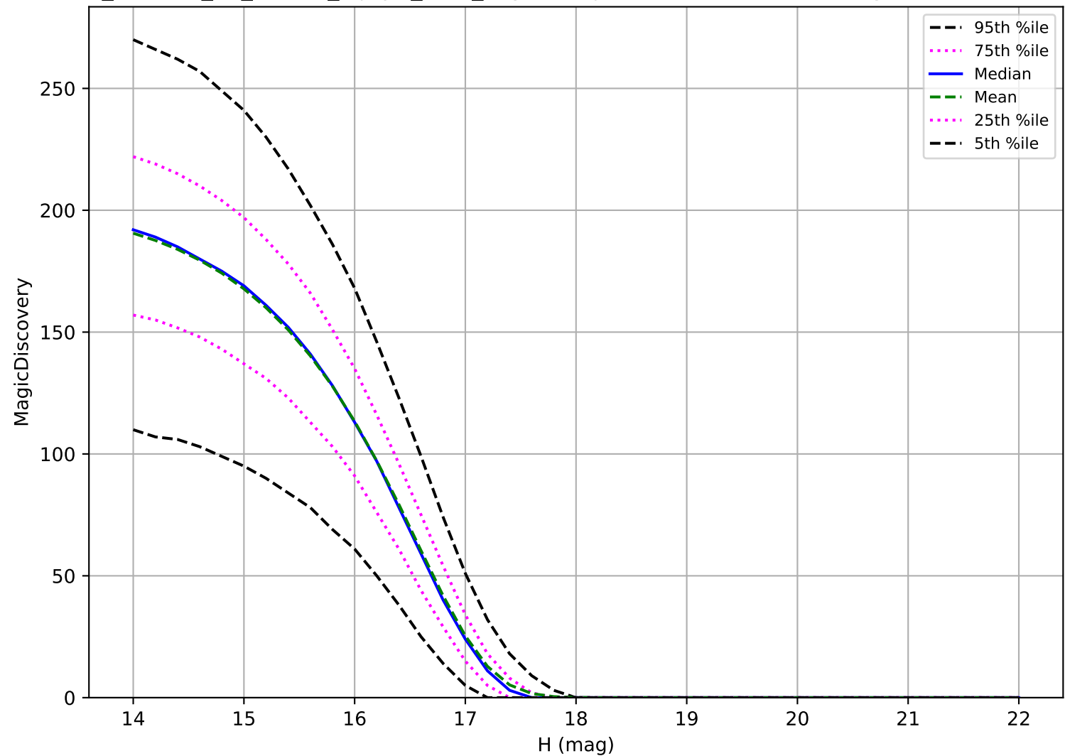
roll_uniform_eh_acc0.2_mjdp0_v3.4_10yrs: Trojan 6 detections in 60 nights detection loss
