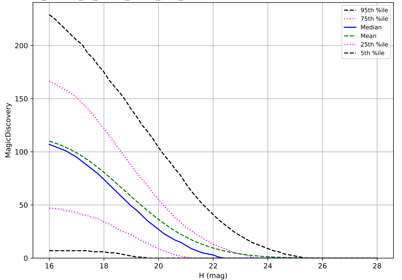
roll_uniform_eh_acc0.2_mjdp0_v3.4_10yrs: PHA 6 detections in 60 nights detection loss
