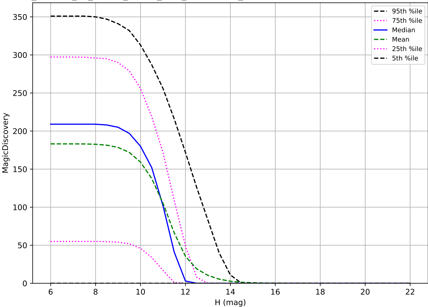
roll_uniform_eh_acc0.2_mjdp0_v3.4_10yrs: OCC_r20 6 detections in 60 nights detection loss
