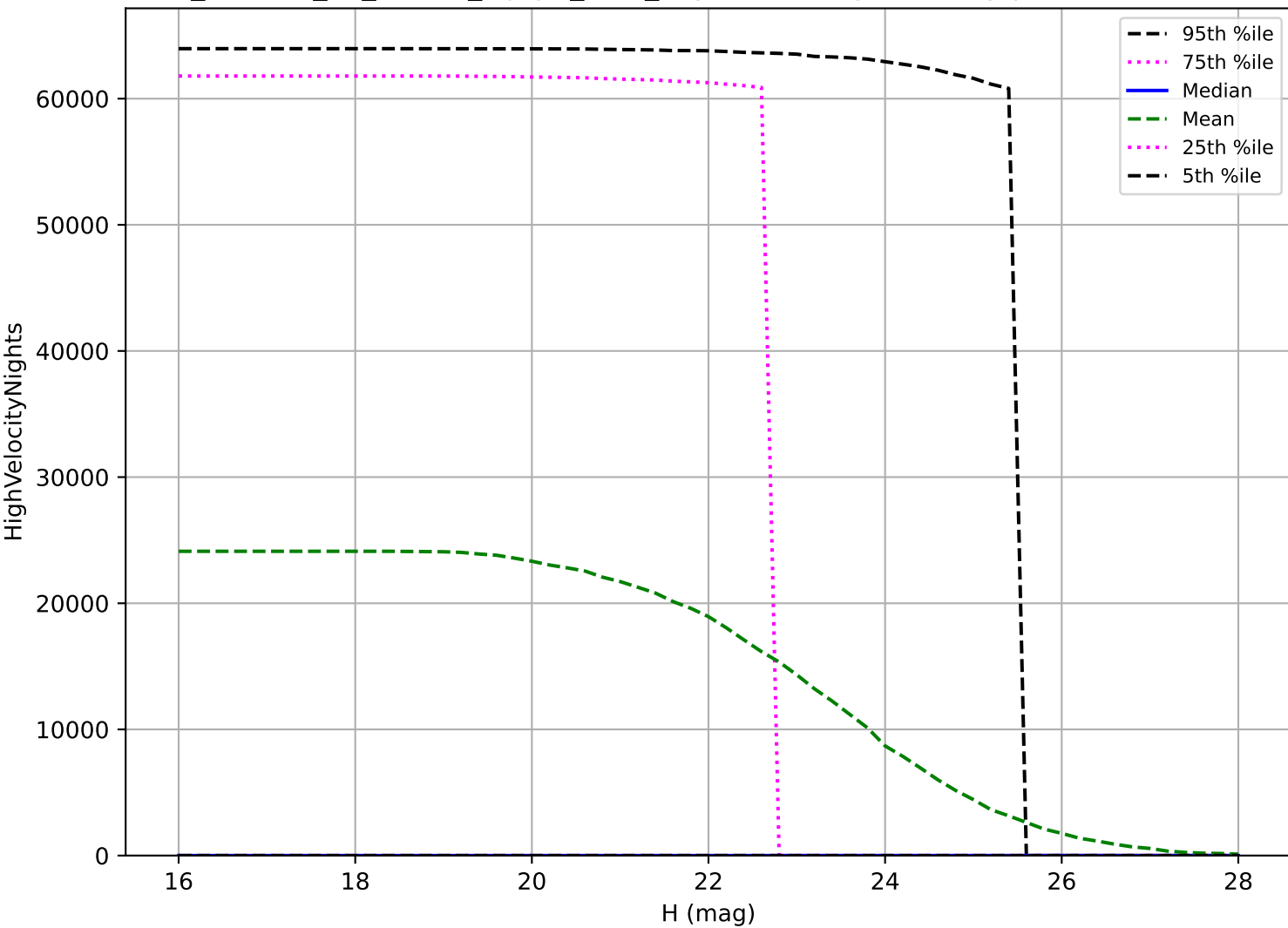
roll_uniform_eh_acc0.2_mjdp0_v3.4_10yrs: PHA High velocity pair detection loss
