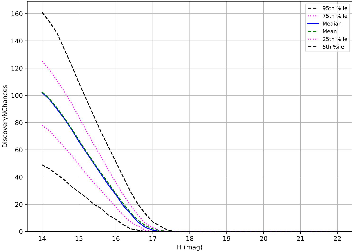
roll_uniform_eh_acc0.2_mjdp0_v3.4_10yrs: Trojan 3 pairs in 15 nights detection loss
