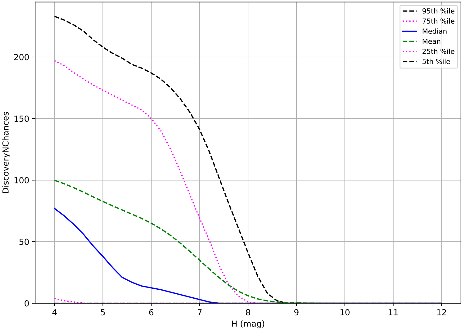
roll_uniform_eh_acc0.2_mjdp0_v3.4_10yrs: TNO 3 pairs in 15 nights detection loss
