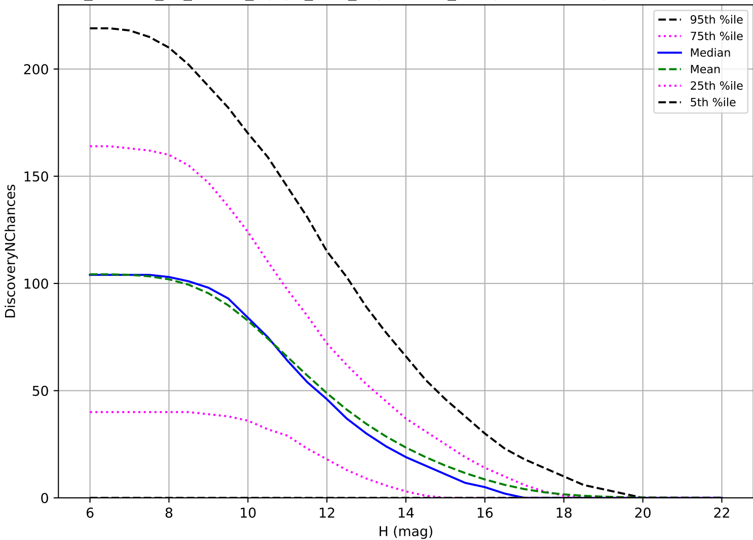
roll_uniform_eh_acc0.2_mjdp0_v3.4_10yrs: OCC_r5 3 pairs in 15 nights detection loss
