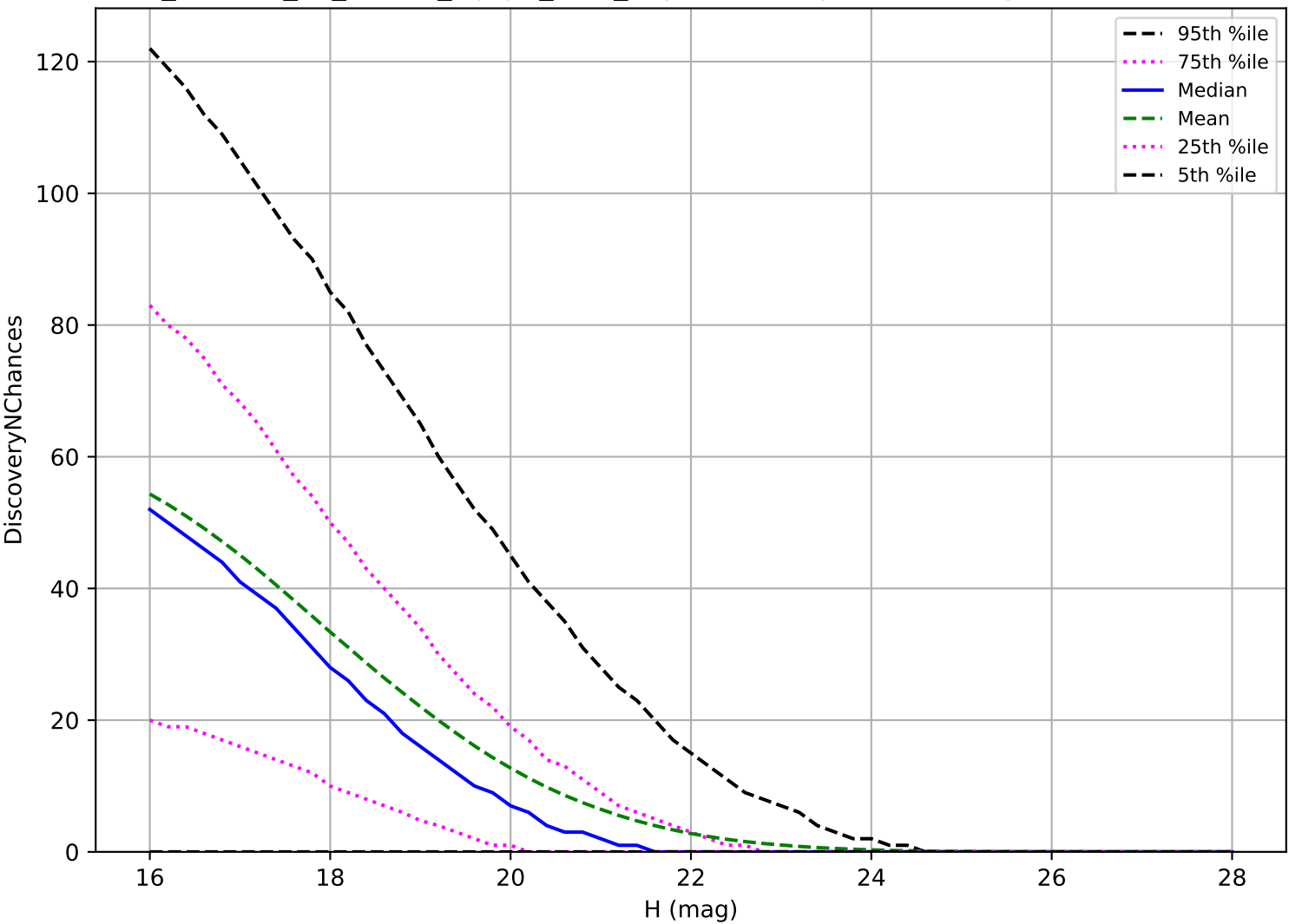
roll_uniform_eh_acc0.2_mjdp0_v3.4_10yrs: NEO 3 pairs in 15 nights detection loss
