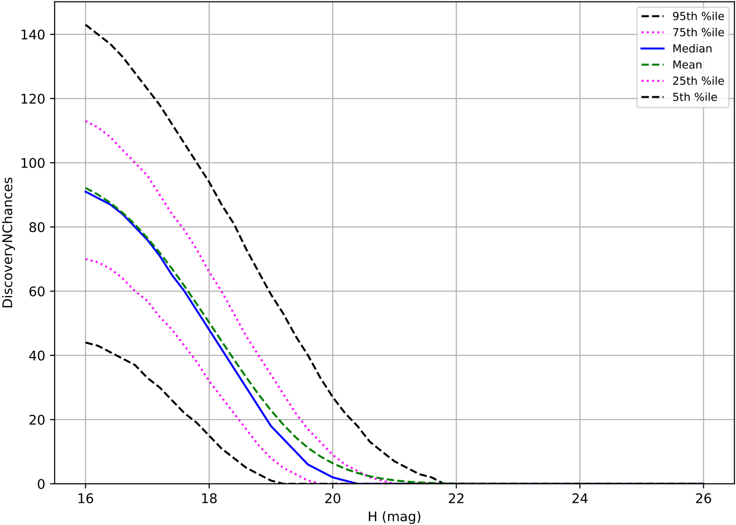
roll_uniform_eh_acc0.2_mjdp0_v3.4_10yrs: MBA 3 pairs in 15 nights detection loss
