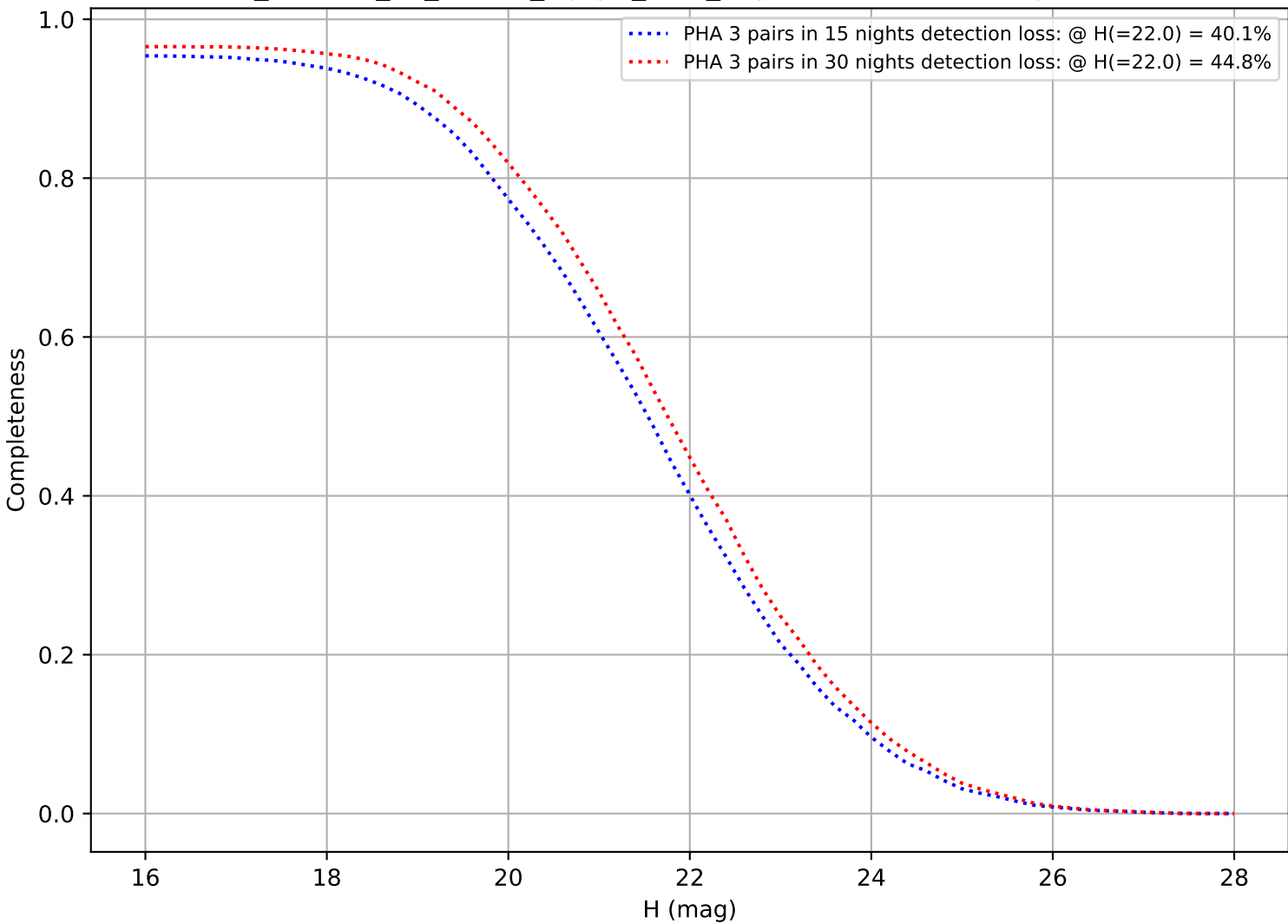
roll_uniform_eh_acc0.2_mjdp0_v3.4_10yrs: DifferentialCompleteness
