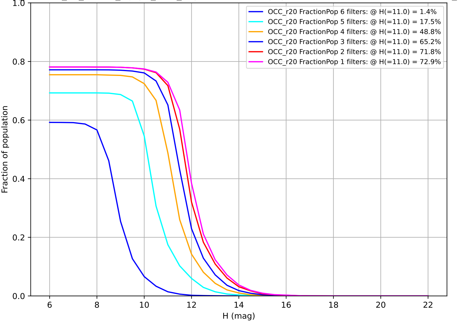
roll_uniform_eh_acc0.2_mjdp0_v3.4_10yrs: Fraction of population with colors in X filters OCC_r20
