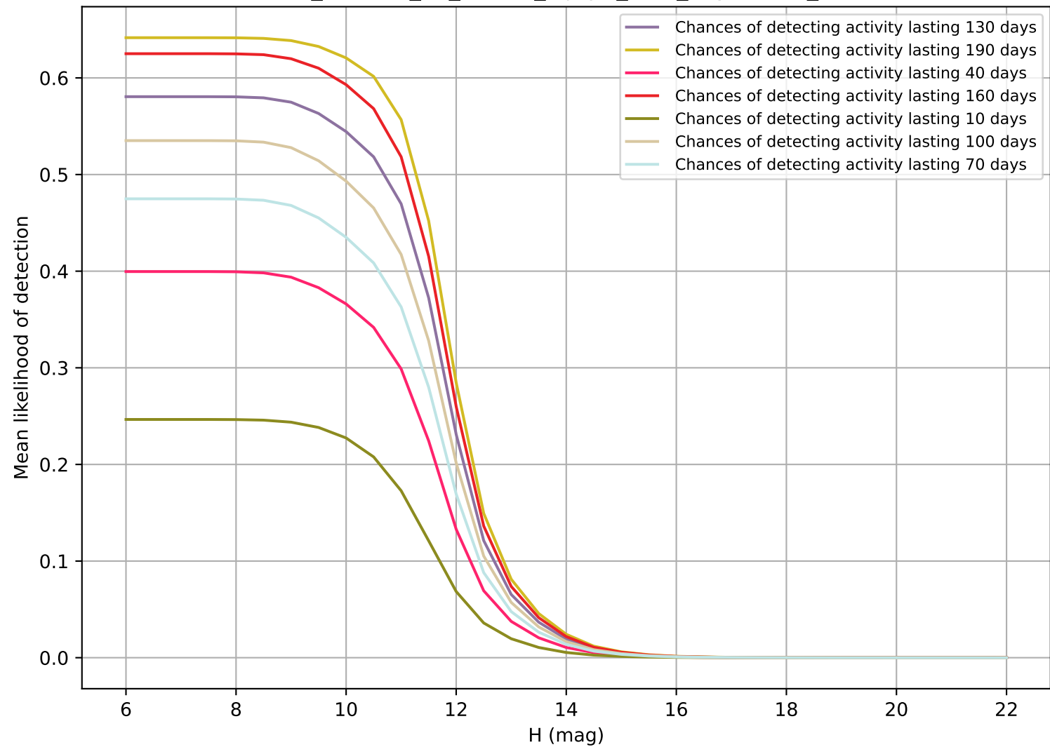
roll_uniform_eh_acc0.2_mjdp0_v3.4_10yrs OCC_r20
