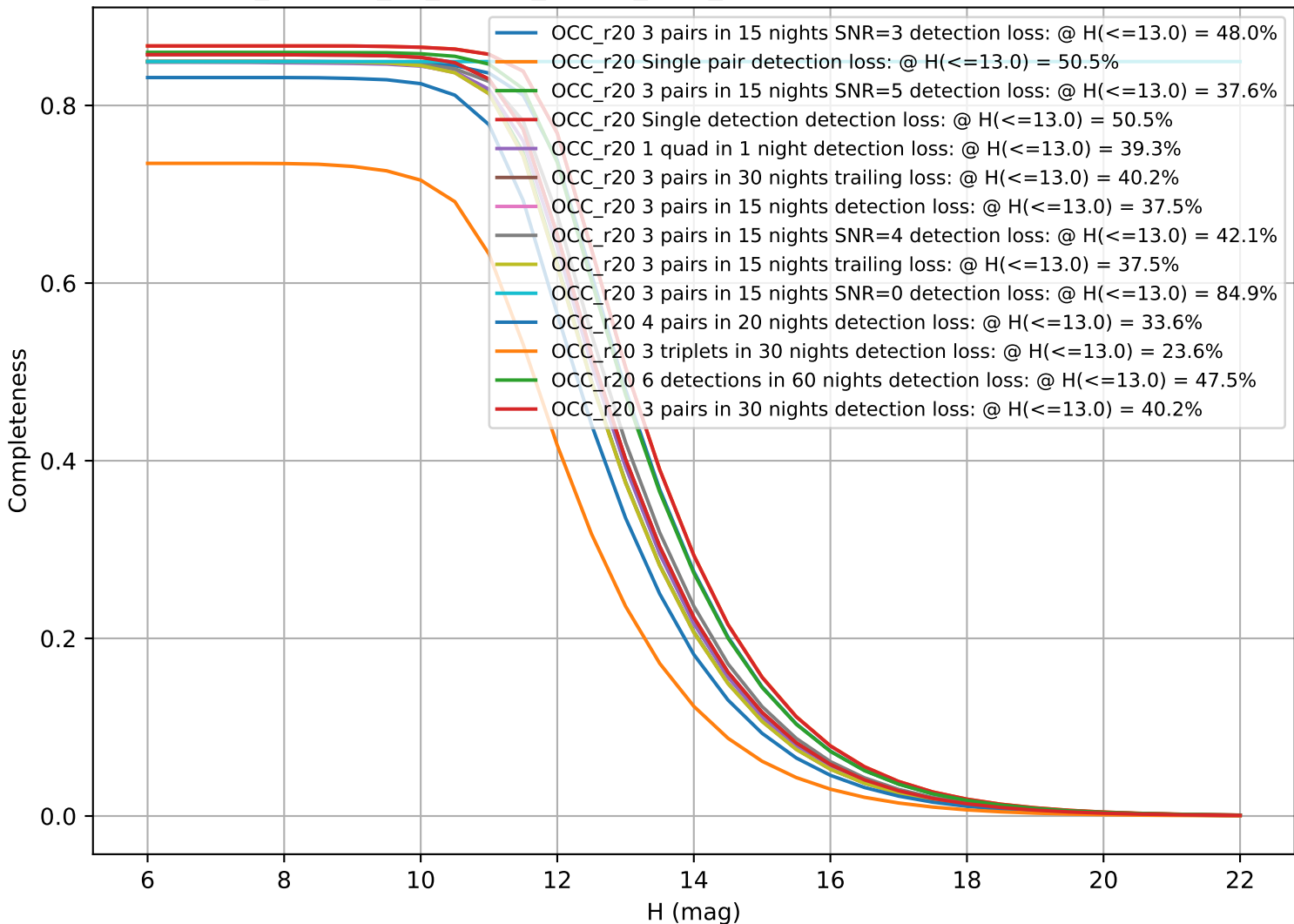
roll_uniform_eh_acc0.2_mjdp0_v3.4_10yrs: CumulativeCompleteness
