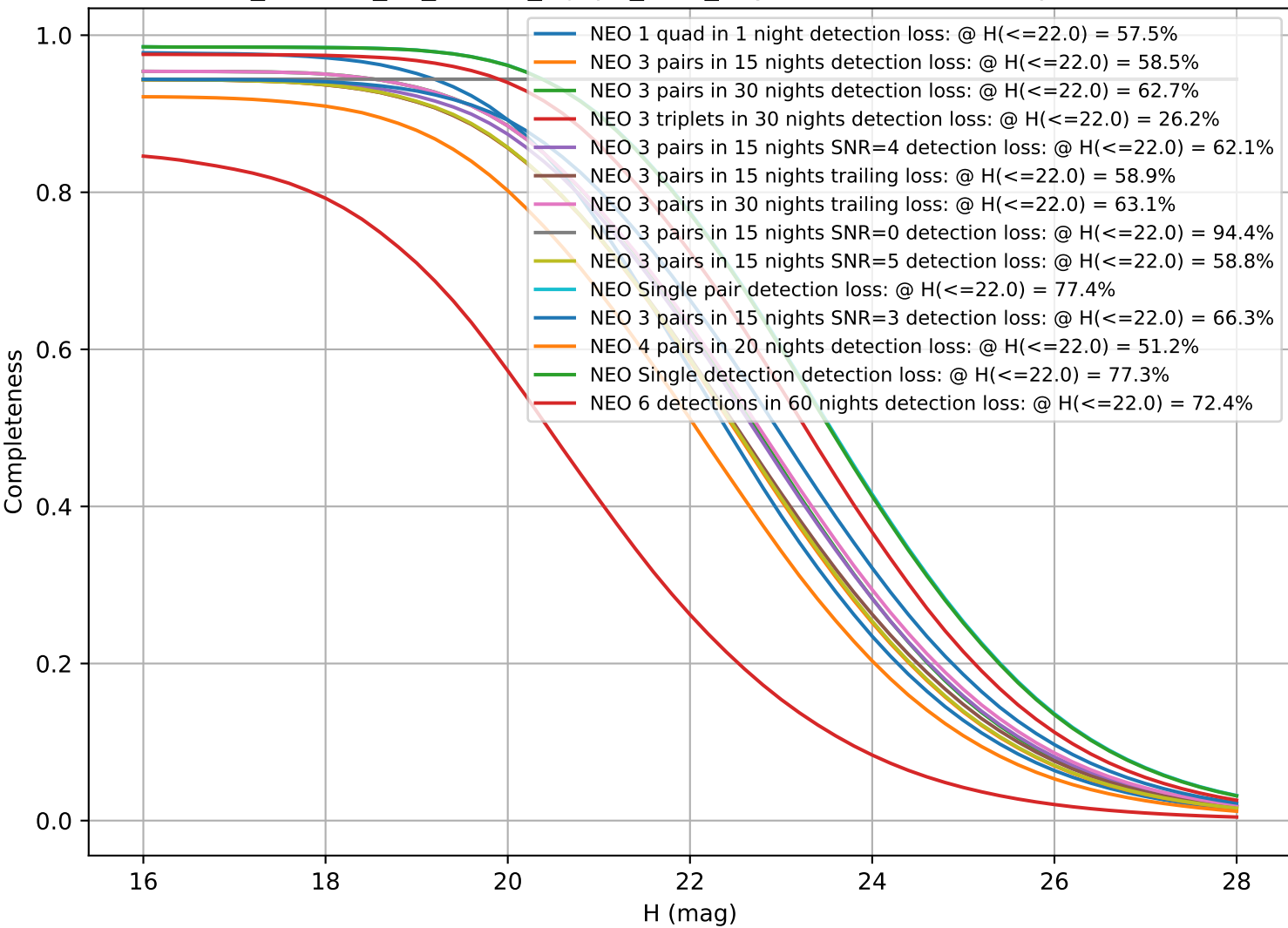
roll_uniform_eh_acc0.2_mjdp0_v3.4_10yrs: CumulativeCompleteness
