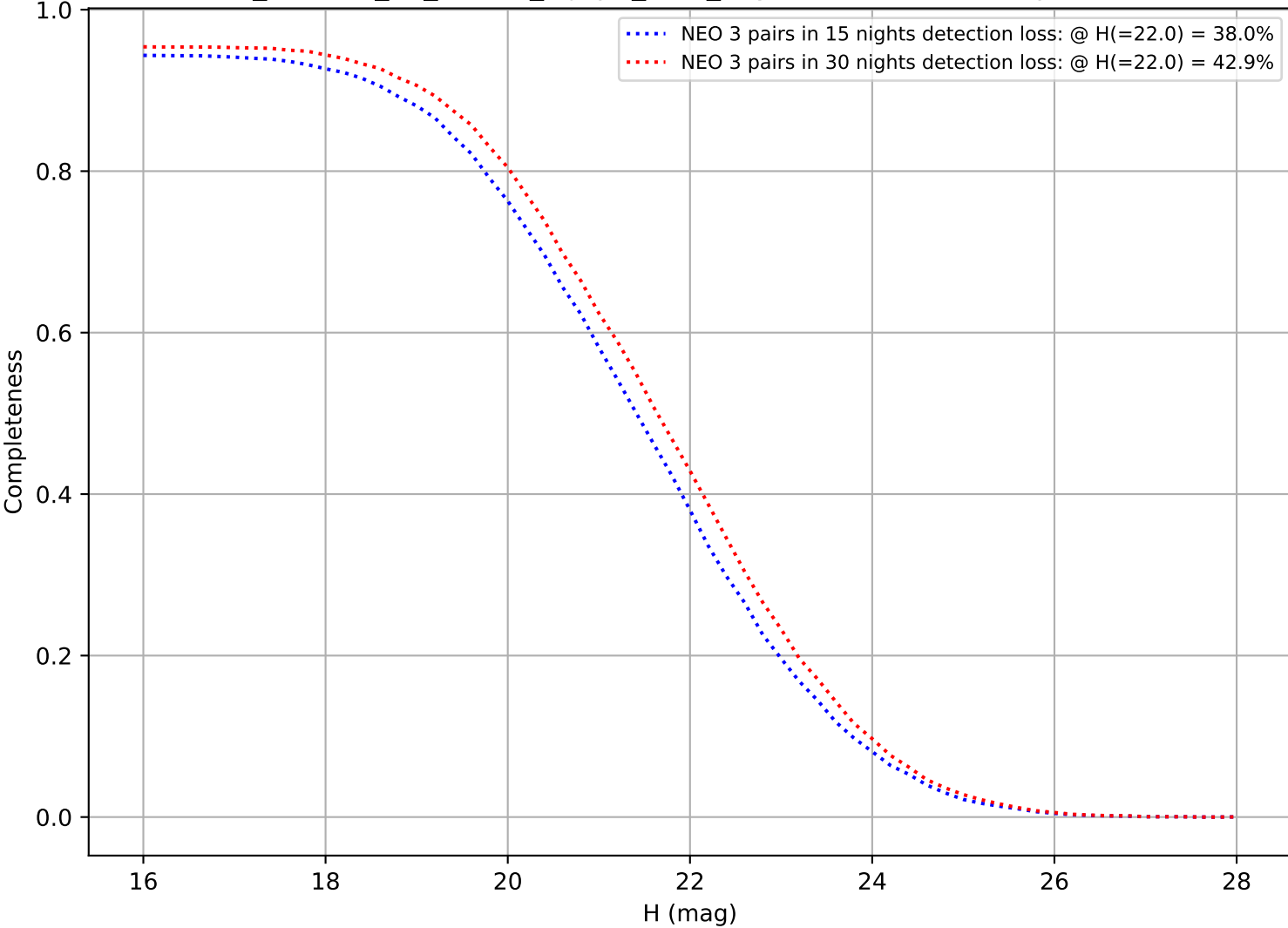
roll_uniform_eh_acc0.2_mjdp0_v3.4_10yrs: DifferentialCompleteness
