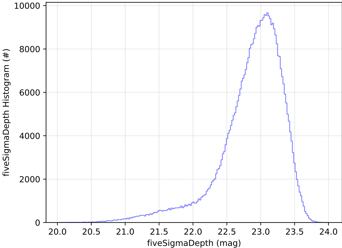
roll_uniform_eh_acc0.2_mjdp0_v3.4_10yrs z: fiveSigmaDepth Histogram
